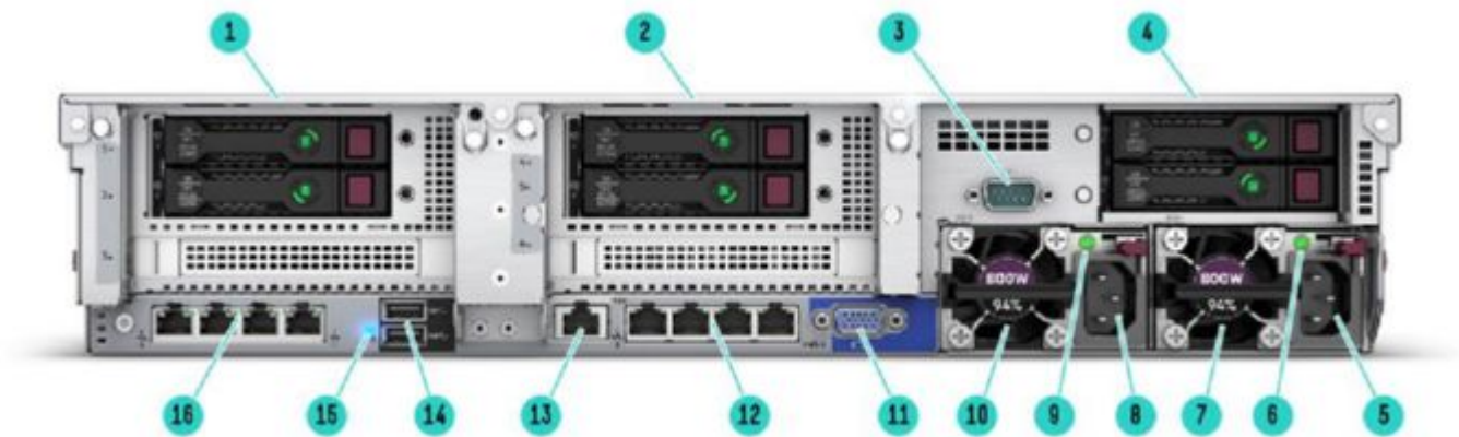
HPE ProLiant DL385 Gen10 Server - Rear View With optional FlexLOM, Rear drives and Serial port shown
