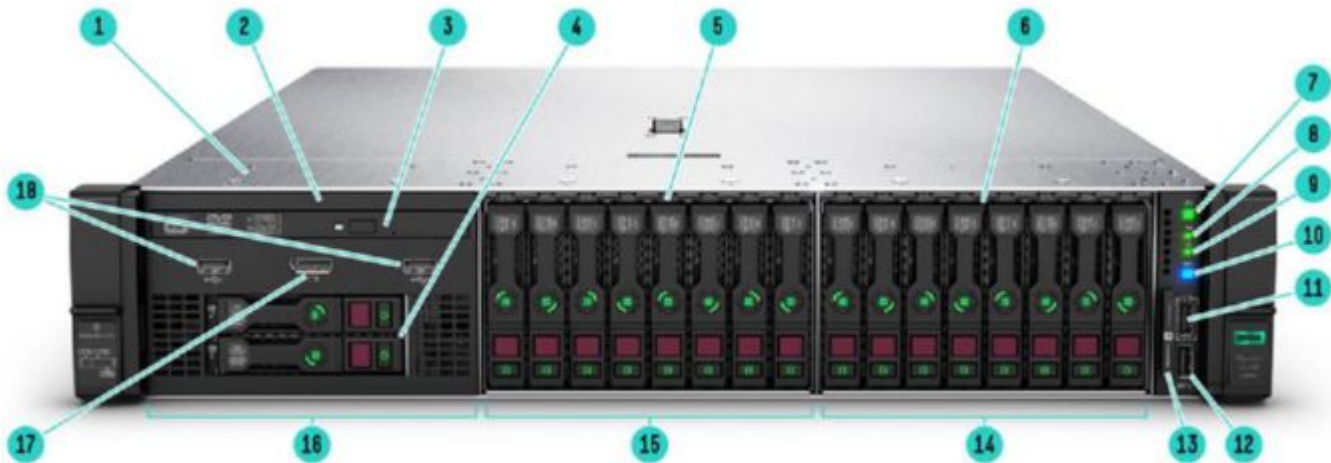
HPE ProLiant DL385 Gen10 Server - Front View
