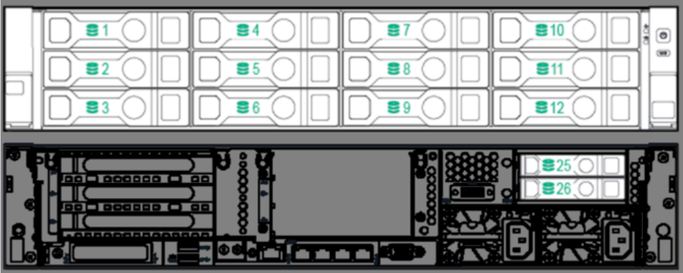
12 LFF + 2 rear SFF hot-plug drive model
