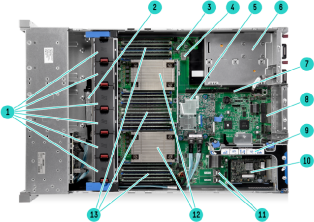
Internal View
