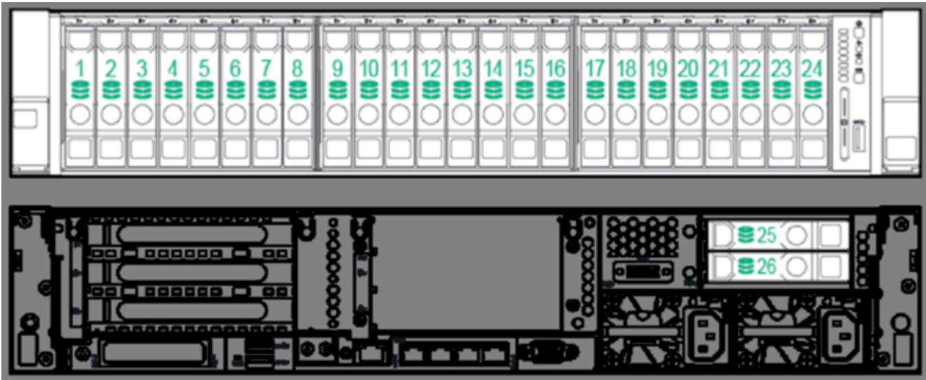
24 SFF + rear 2 SFF hot-plug drive model
