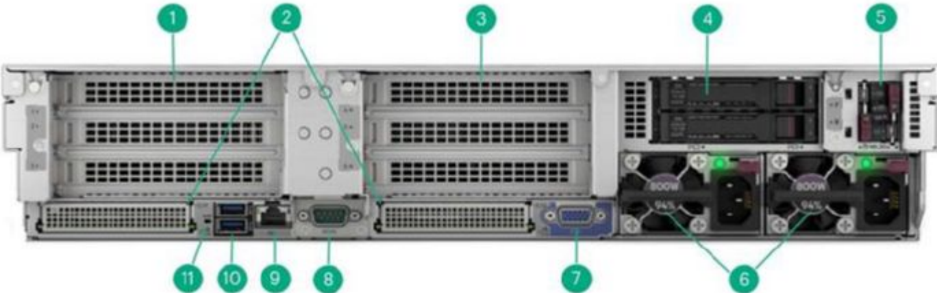
Rear View - Standard for all DL380 Gen11
