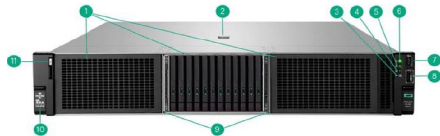
Front View -12EDSFF chassis shown
