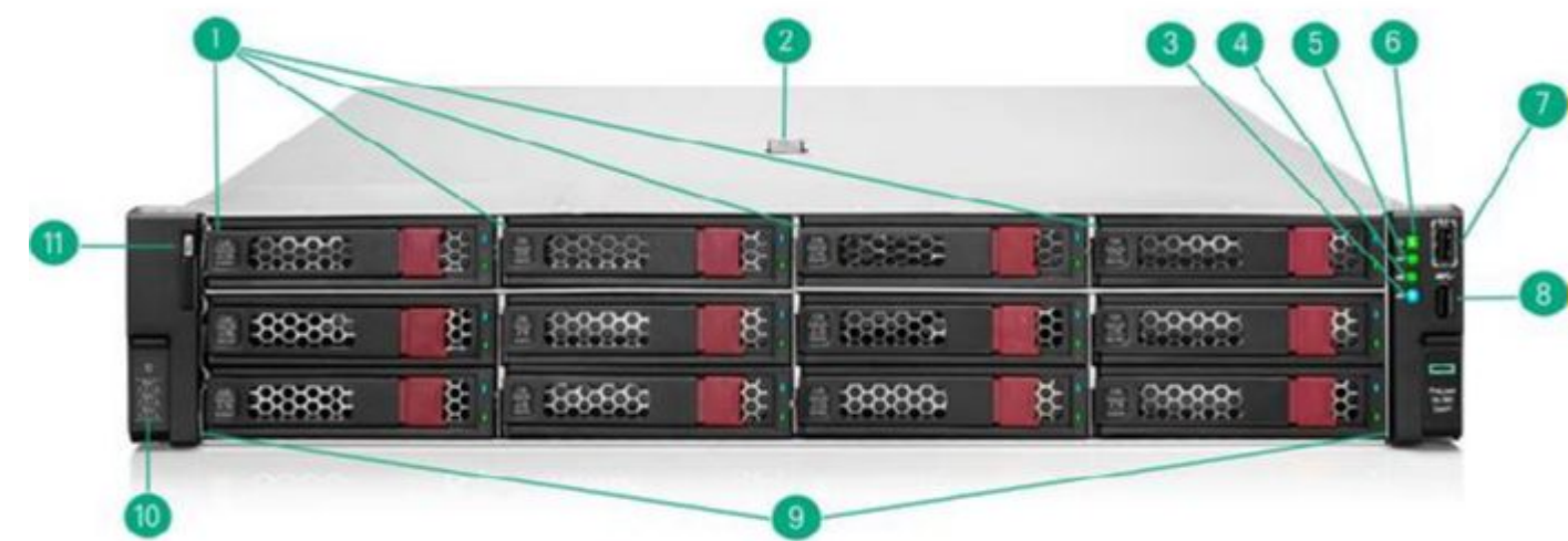
Front View - 12LFF chassis shown
