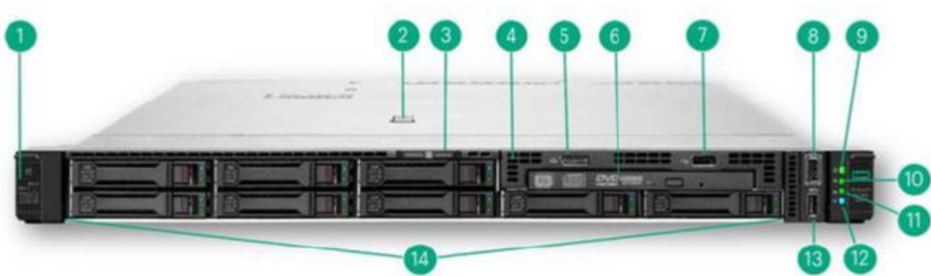
8 SFF Front View- 8 SFF + optional Universal Media Bay, optical drive, DisplayPort, USB2.0 and SAS drives shown
