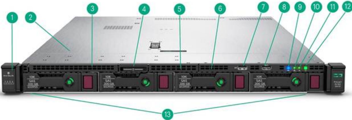
4 LFF Front View - Standard 4 LFF shown
