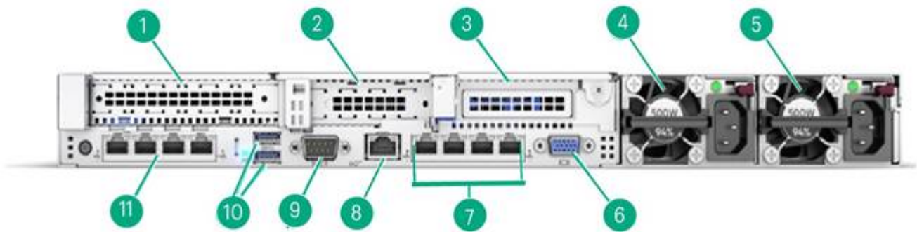
Rear View - Standard for all DL360 Gen10
