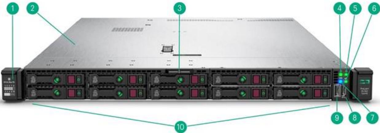
Premium 10SFF NVMe Front View
