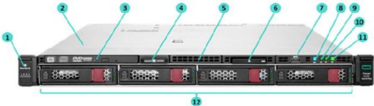
4 LFF Front View - 4 LFF + Optional Systems Insight Display (SID), optical drive and SAS drives shown
