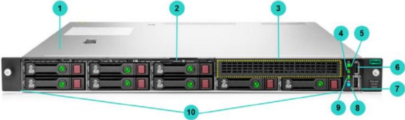
8 SFF chassis - Front View
